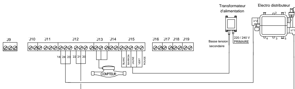
Schéma n° XIV - " Raccordements version simplex "
