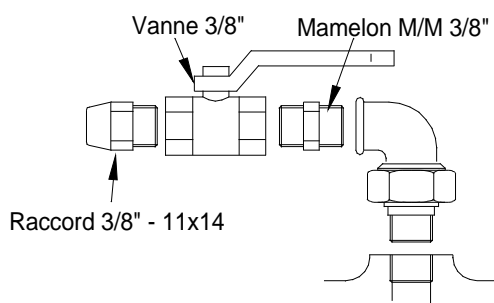
Schéma n° XI - " Raccordement aspiration "
