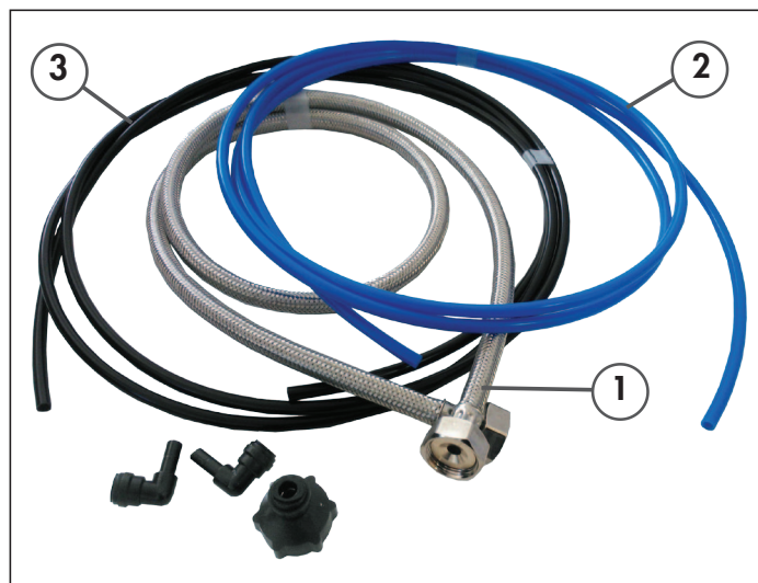
Fig.1: Example overview of the hose connection kit 1, (1) feed water hose, (2) pure water hose, (3) concentrate hose
