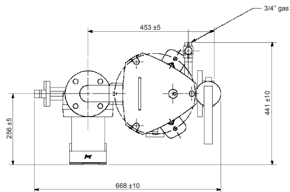
DESLUDGING UNIT 10/20
